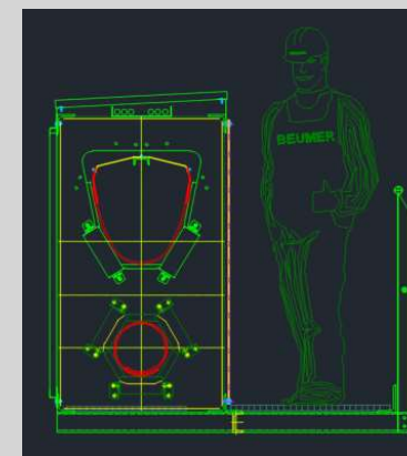
U-shaped belt conveyor
